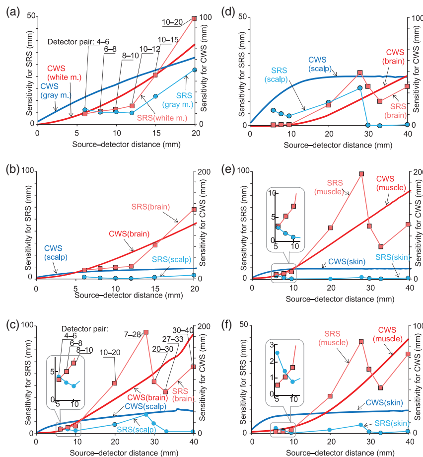
Fig. 4 Measurement sensitivity of SRS and CWS for each model, each layer, and each detector pair. Symbols (a)–(f) correspond to Fig. 1. Detector pair of (b) is the same as (a), and pairs of (d)–(f) are shown in (c).
